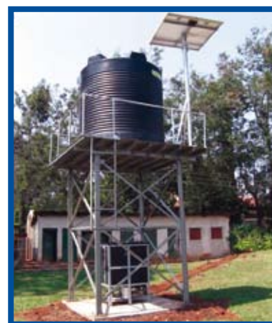
Water supply system at St Francis Hospital.
